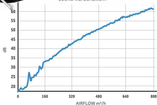
SOUND MEASUREMENT
