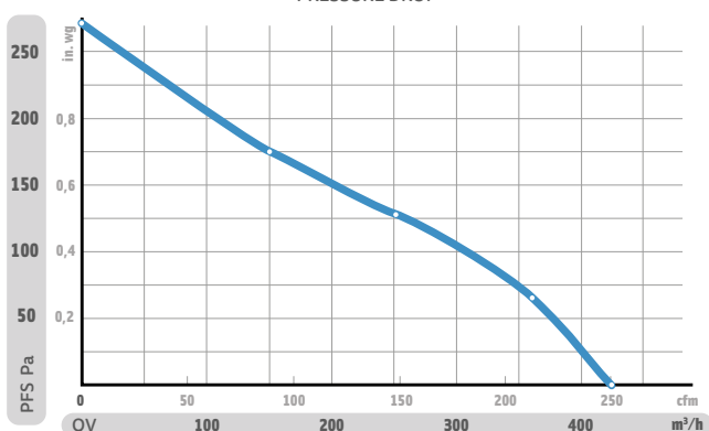
PRESSURE DROP
