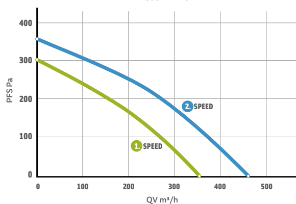
PRESSURE DROP
