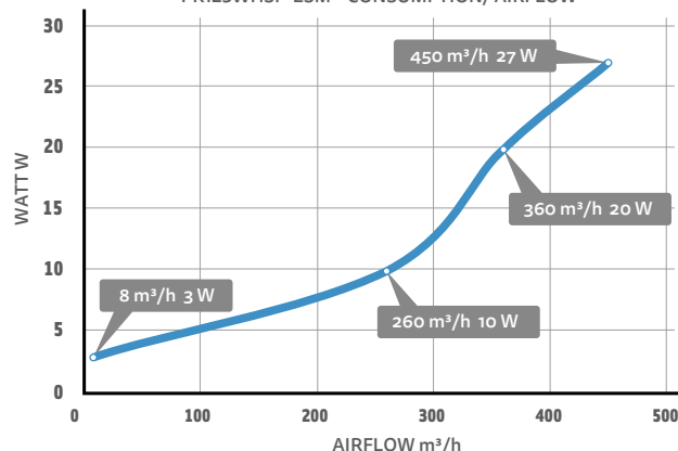
PK125WHSP-ESM - CONSUMPTION/ AIRFLOW
