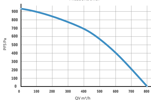
PRESSURE DROP
